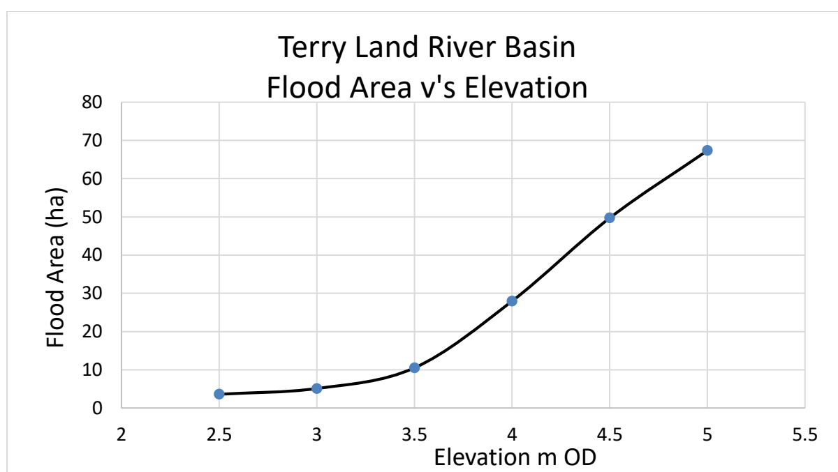
Figure 15 Flood Area – Elevation Relationship in the Terryland Floodplain
