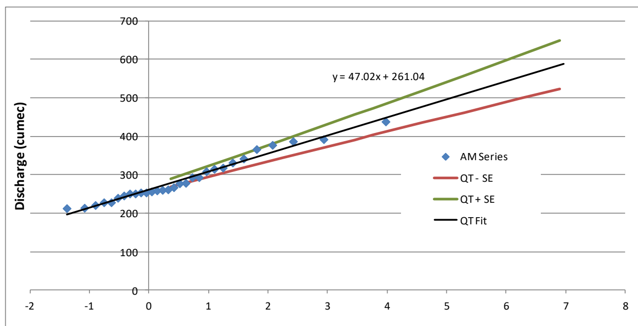
Figure 7 EV1 Fit to Annual Maxima Estimated Flood Flow Series at Dangan including the statistical error (67% confidence) limits
