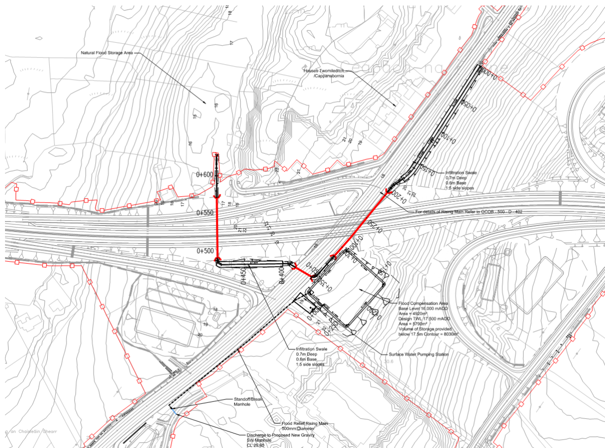
Figure 14 Flood relief mitigation measures for Twomileditch / N17 Tuam Road area
