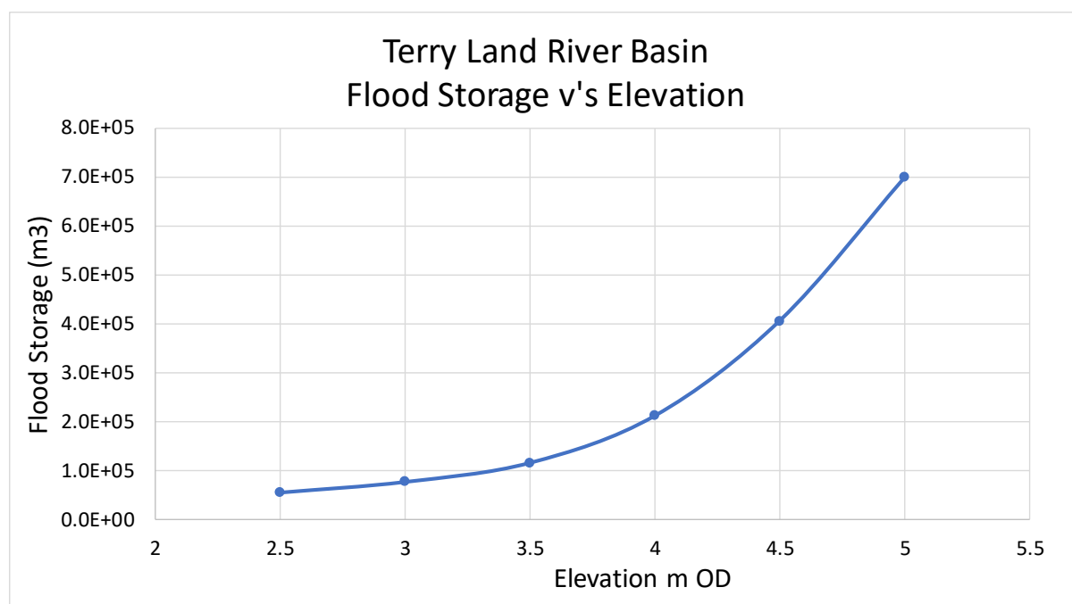
Figure 16 Flood Storage – Elevation Relationship in the Terryland Floodplain
