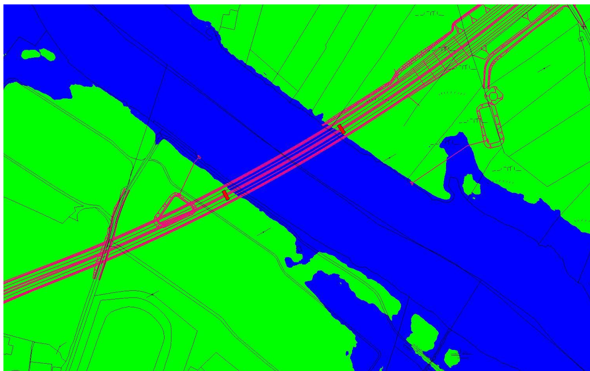
Figure 7 Flood inundation at River Corrib crossing for the 1000 year flood event
