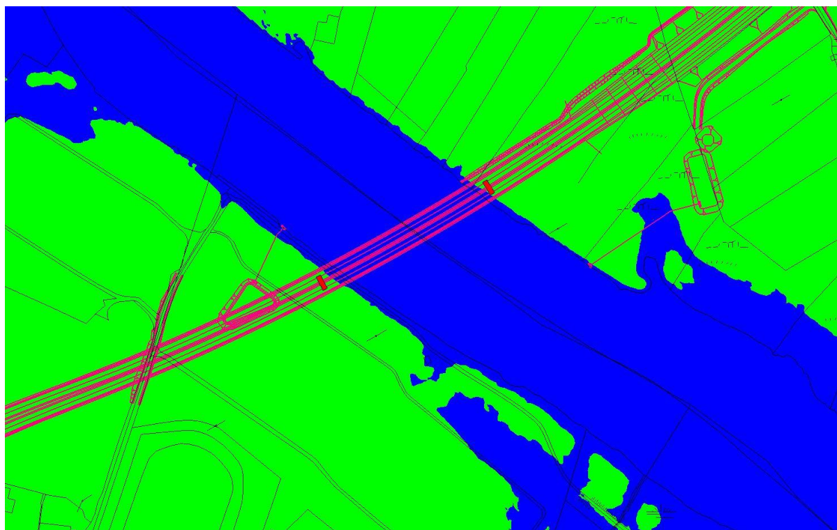
Figure 8 Flood inundation at River Corrib crossing for the 100 year with Climate Change flood event
