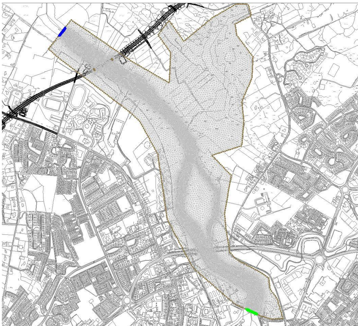
Figure 8 2-D model domain
