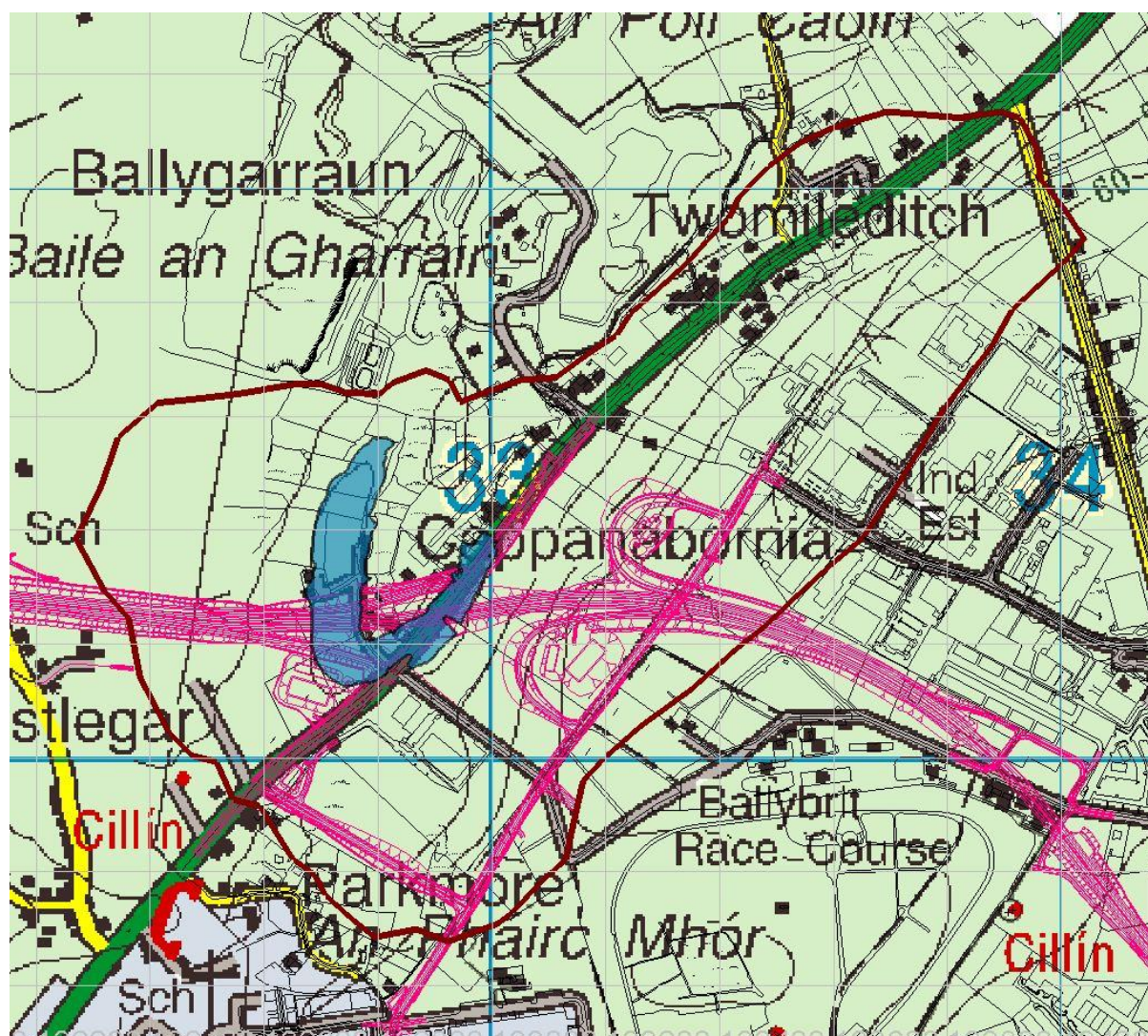
Figure 13 Twomileditch / N17 Tuam Road drainage catchment and the flood risk lands by the 18.5m OD Contour and the proposed road alignment overlaid.
