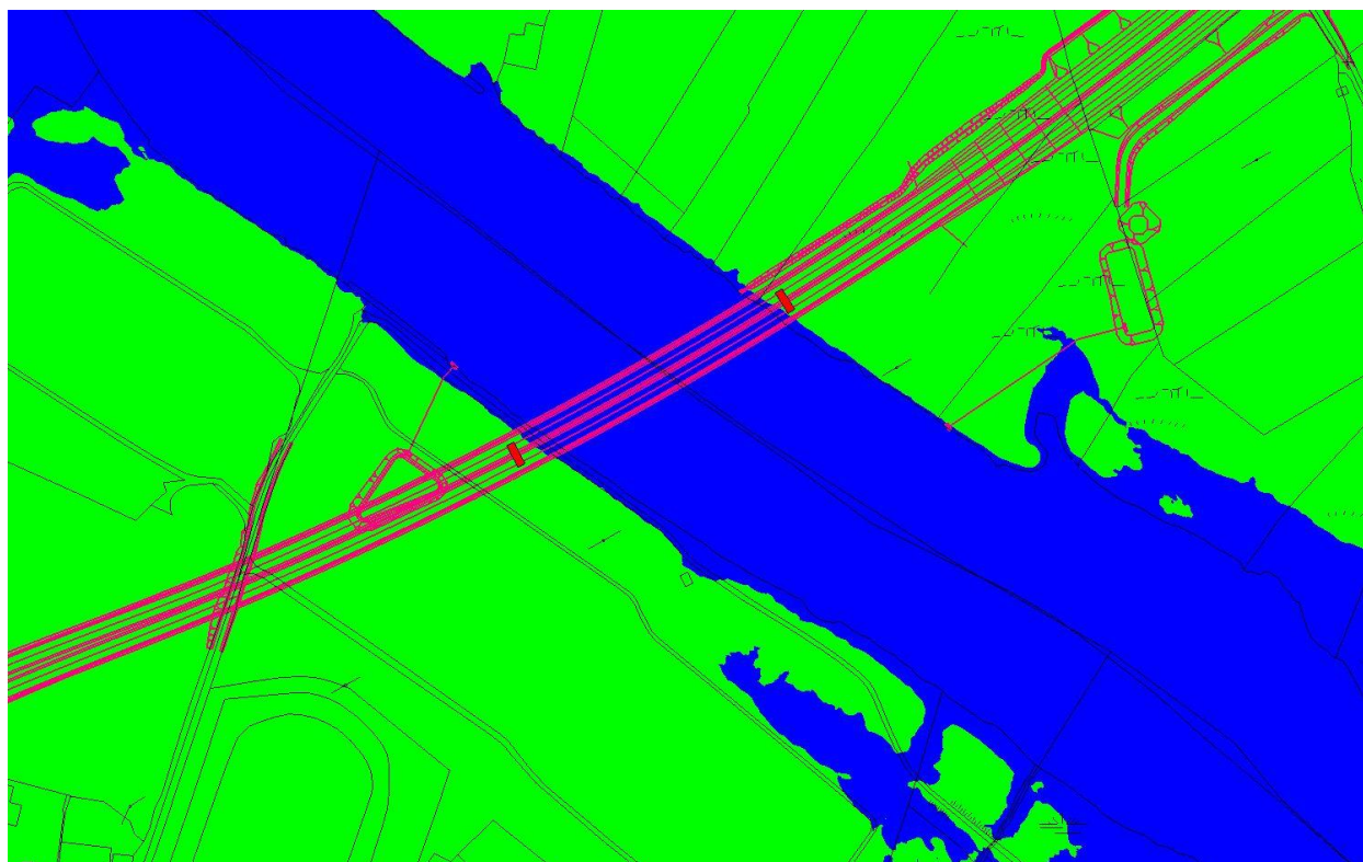
Figure 6 Flood inundation at River Corrib crossing for the 100 year flood event
