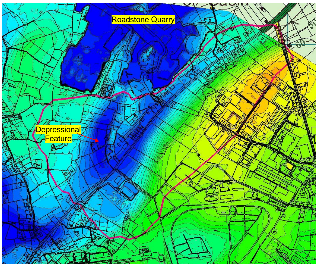
Figure 12 Twomileditch / N17 Tuam Road drainage catchment and 2m contours showing depressional feature that is subject to flooding.
