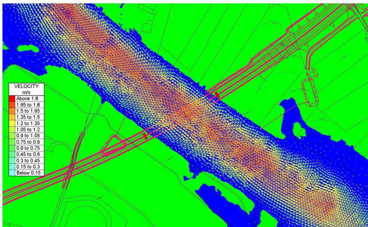
Figure 9 River Corrib velocity plot of 100 year with CC peak flow at proposed bridge crossing
